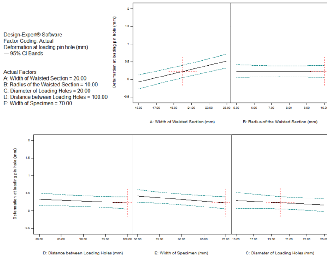
Figure 4-10, Main effect plot for elongation in the loading pinhole.
