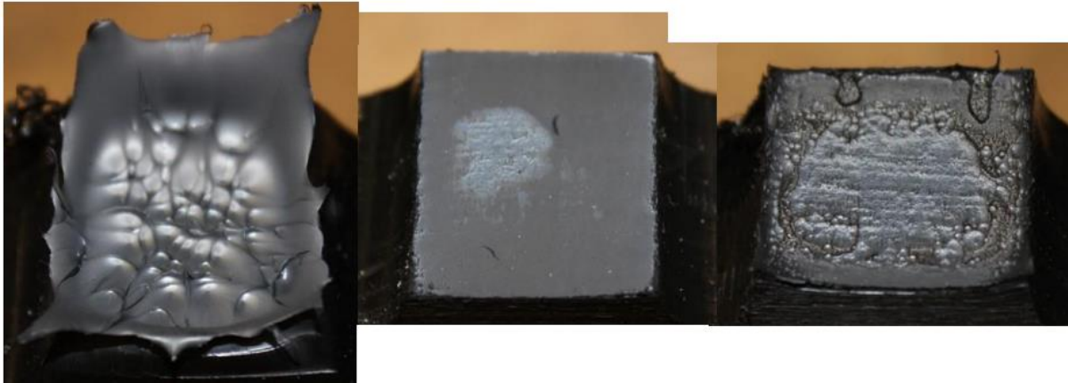
Figure 3-2, from left ductile, brittle and mixed failure mode according to WIS 4-32-08
