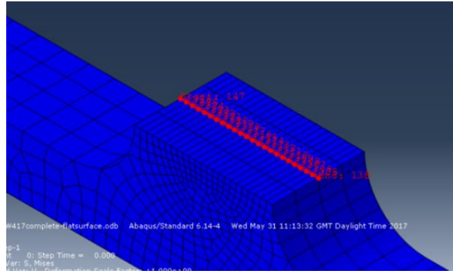
Figure 5-5, Triaxiality measurement point locations in the specimens
