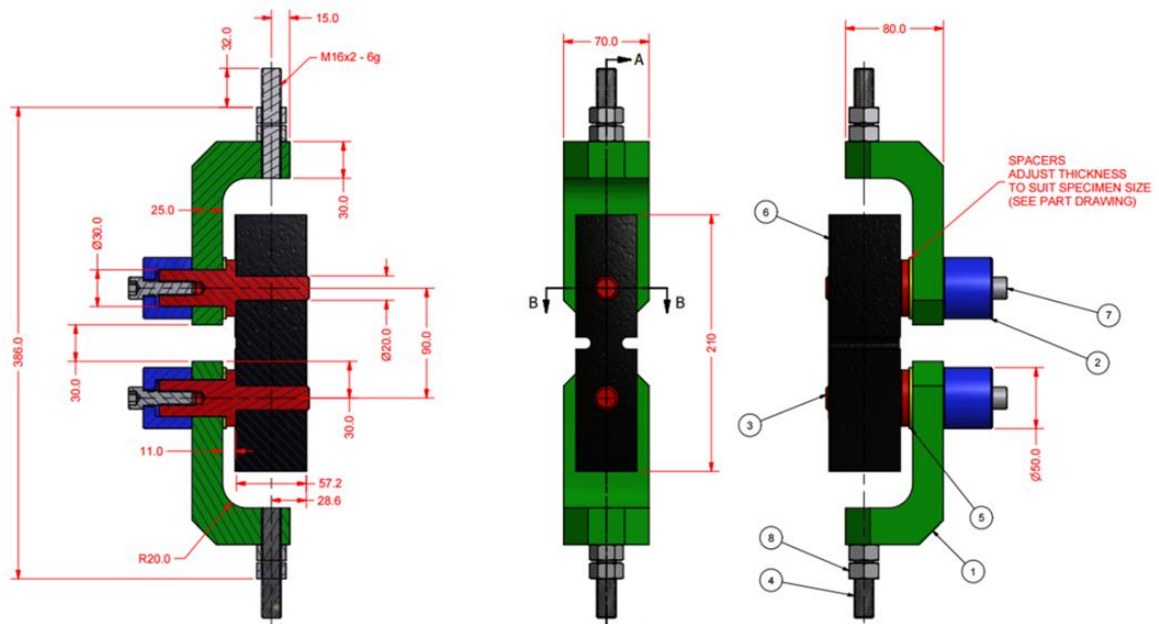
Figure 8-1, Tensile test engineering design for DIC purpose
