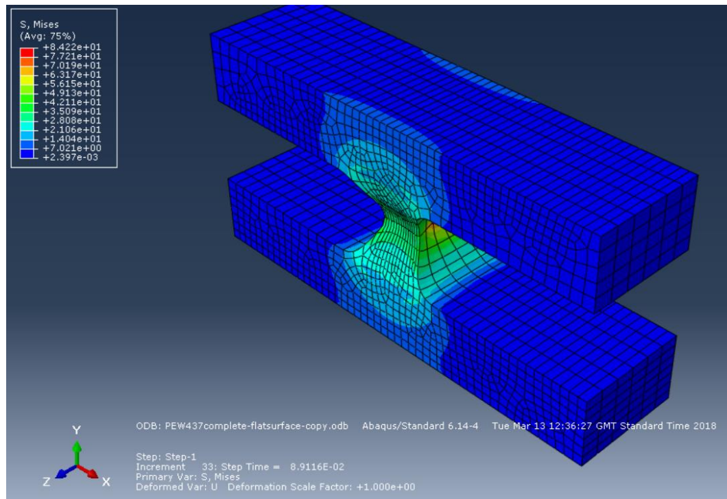
Figure 5-9, later increment of neck development modelling
