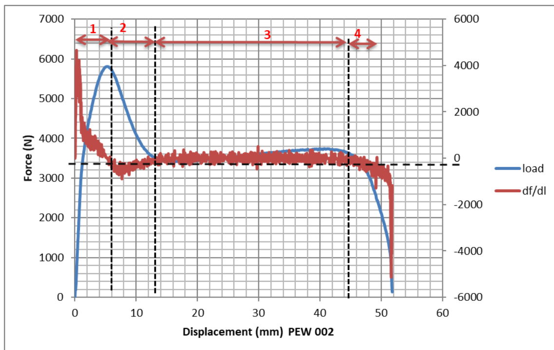
Figure 3-5, Graph shows the force-displacement curve for specimen no PEW002, divided into four regions
