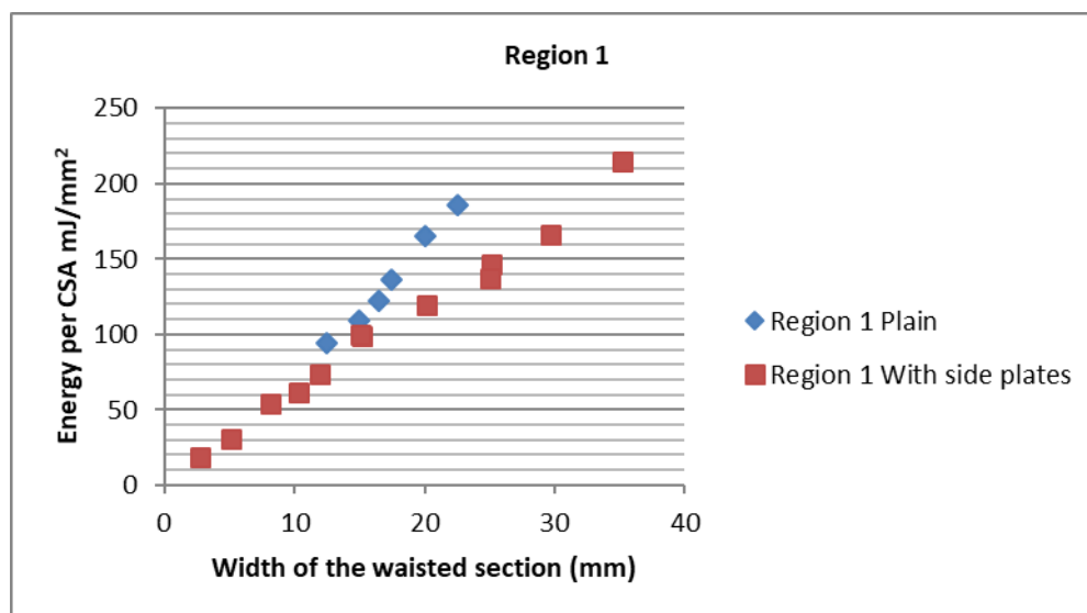
Figure 3-11, Energy per CSA against the width of the waisted section on 15mm thick specimen with and without side plates for Region 1
