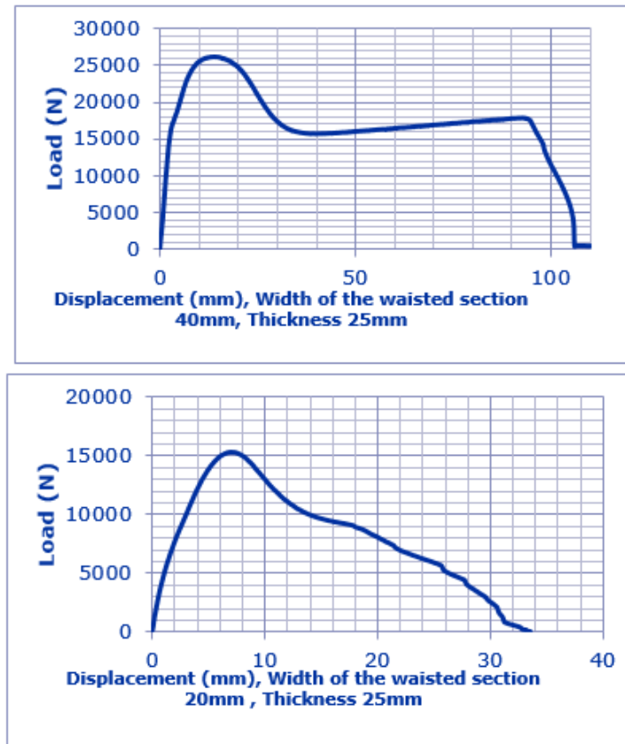
Figure 3-7, Load-displacement for 20mm and 40mm width of the waisted section
