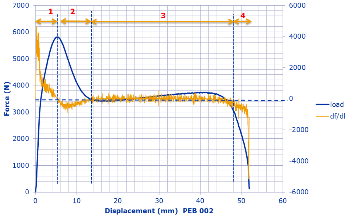
Figure 4-3, Example of a typical Force-Deformation graph
