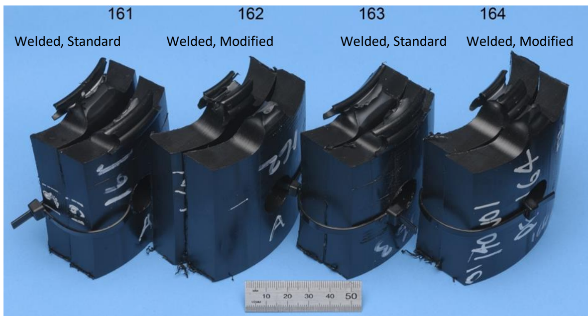
Figure 6-9, From Left, the fracture surface of standard, modified, standard and modified specimen geometry from 140mm OD welded pipe
