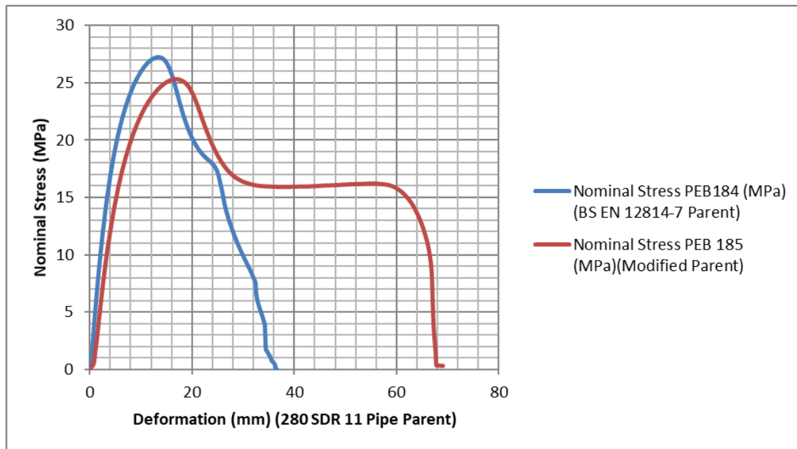
Figure 6-23, Nominal stress-Deformation graph for modified and standard geometry on parent 280mm OD pipe
